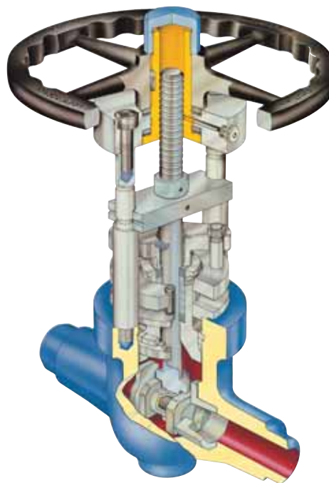
Martyr valve
