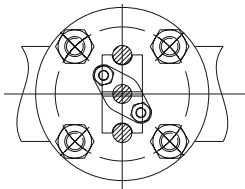
PART SECTION SHOWING CORRECT POSITION OF PILLARS, GLAND ETC.
