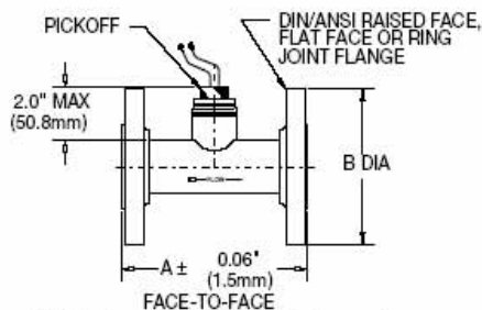
FT Series flowmeter with flanged end connections. Pickoff with flying leads and a 1" NPT spud enclosure connection.
