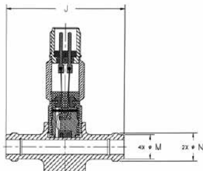
Hose Barb flowmeter with 2-pin MS connector pickoff.
