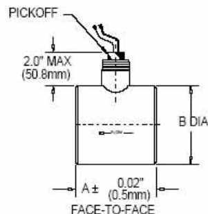
FT Series flowmeter with wafer end connections. Pickoff with flying leads and a 1" NPT enclosure connection on FT-16 and larger.
